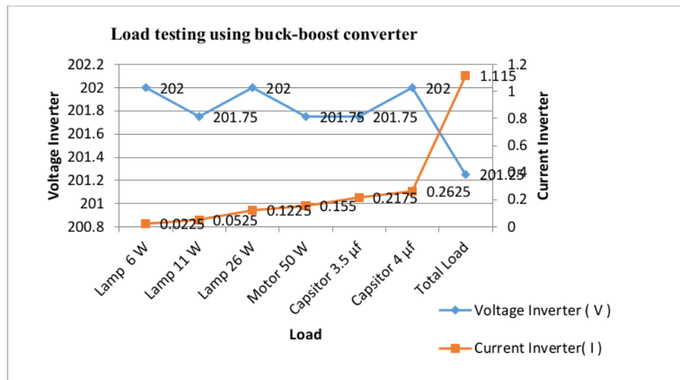
Figure 3. Graph of voltage and current inverter comparison to combined load using buck-boost converter
