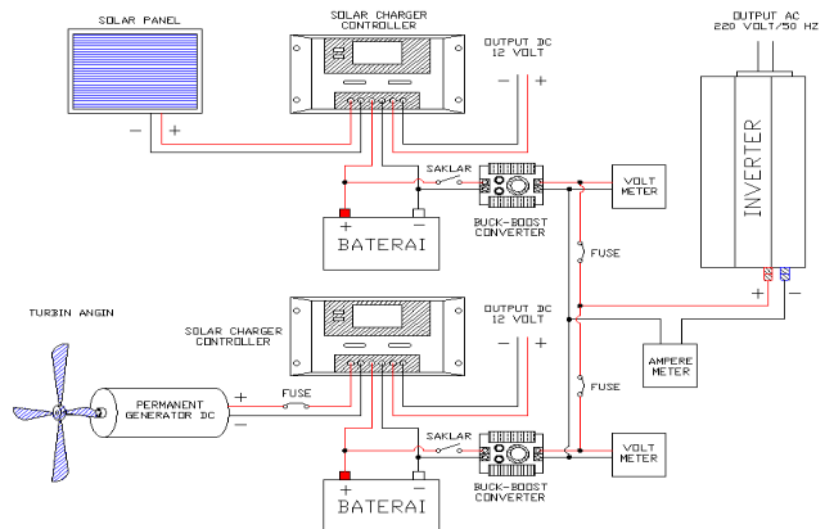
Figure 1. Hybrid generator synchronization series using buck-boost converter
