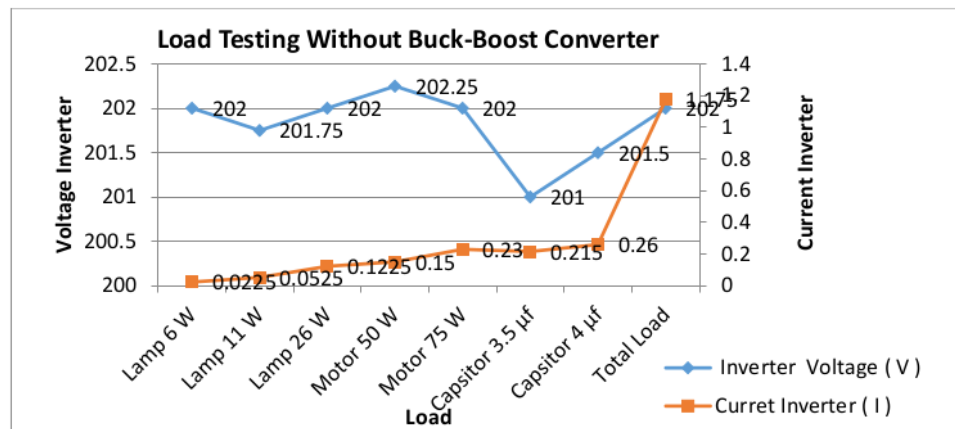
Figure 4. Graph of voltage and current inverter comparison to combined load without using buck-boost converter.
