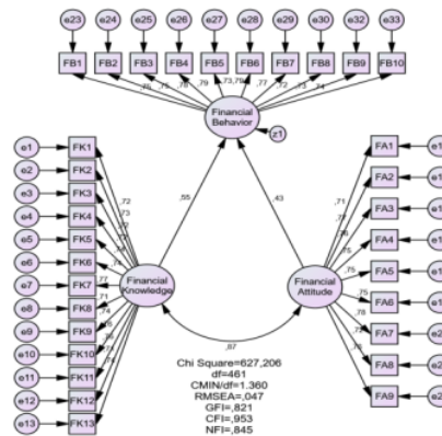
Gambar 1. Hasil Analisis Structural Equation Model (SEM)
