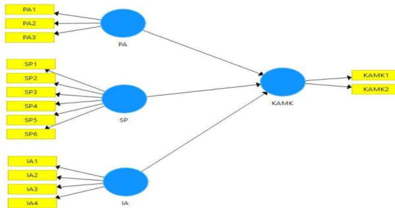
Gambar 2. Model Struktural PLS
