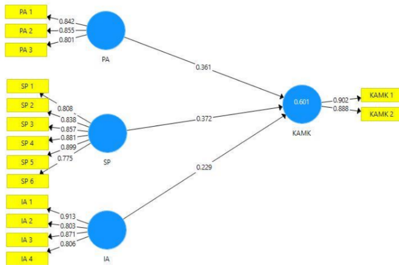
Gambar 3. Output Path Coefficient
