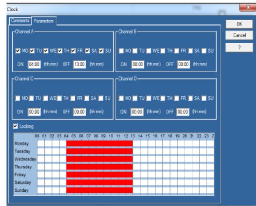
Gambar 5. Jadwal Pengoperasian Pompa Transfer 1
