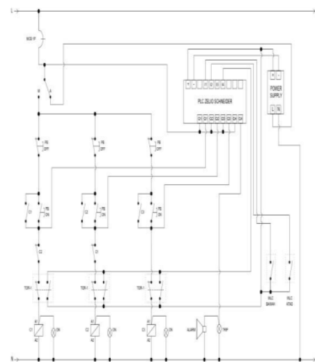
Gambar 2. Diagram wiring otomatis berbasis PLC SR2B121BD
