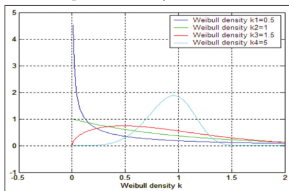
Figure 2: Weibull density for k = variation
