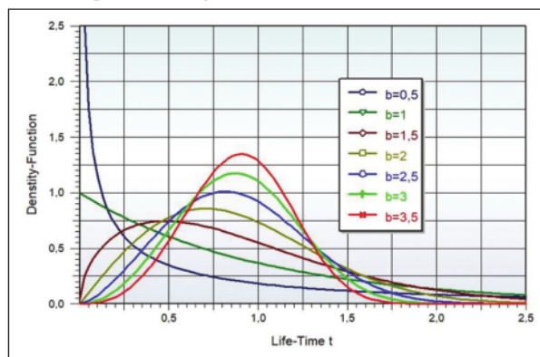
Figure 1: Density function for a = 0 and b = variation
