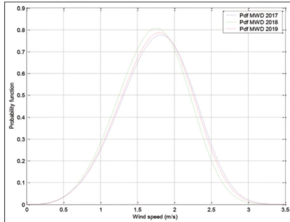
Figure 4: Pdf MWD for 3 years
