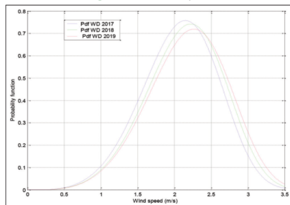
Figure 3: Pdf WD for 3 years
