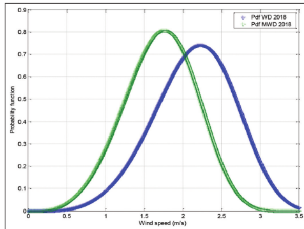
Figure 6: Pdf of WD and MWD for 2018
