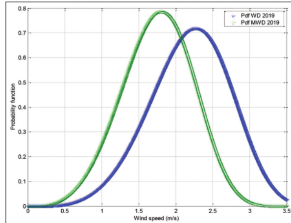
Figure 7: Pdf of WD and MWD for 2019
