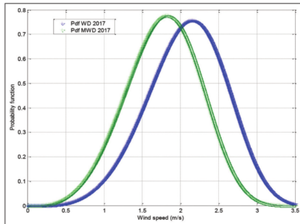
Figure 5: Pdf of WD and MWD for 2017
