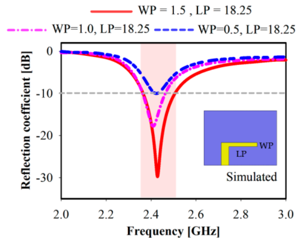
Figure 6. Simulated different patch widths reflection coefficient.
