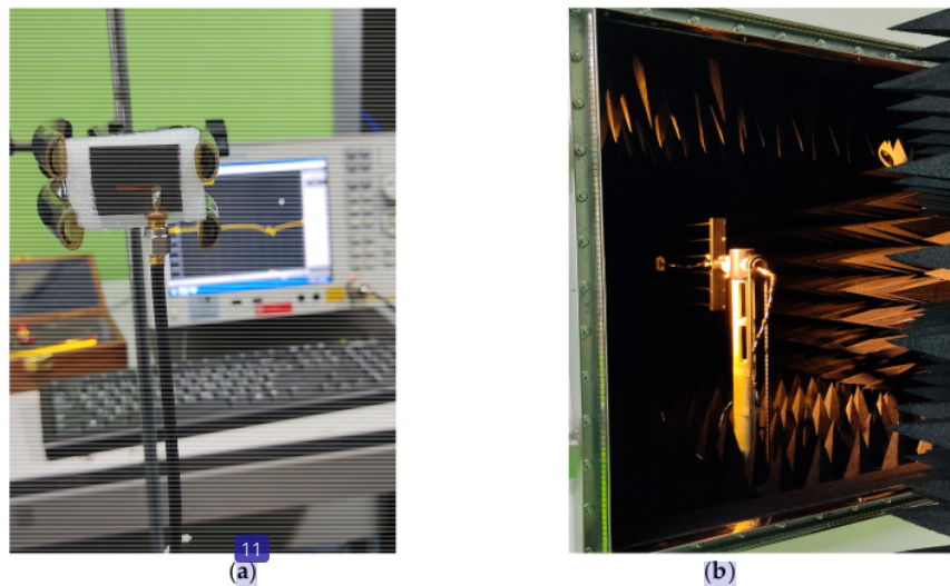
Figure 11. Measurement setup: (a) S11, (b) radiation pattern.
