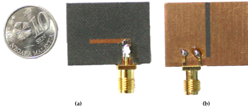
Figure 2. Fabricated prototype: (a) patch, (b) backside ground.
