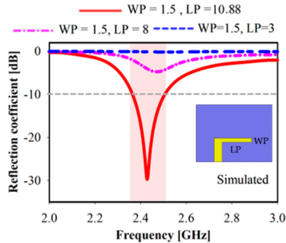
Figure 5. Simulated different patch's length reflection coefficient.
