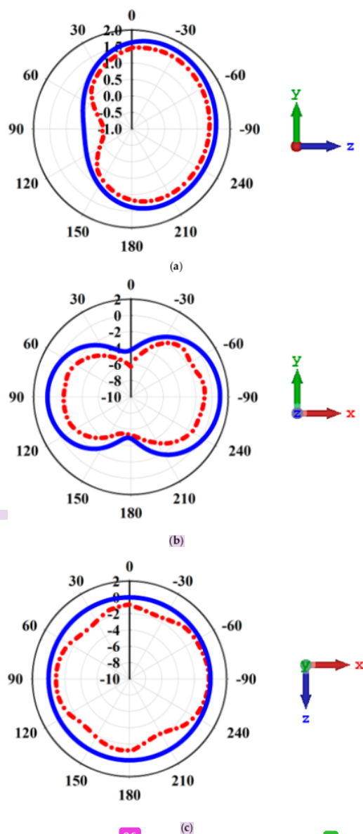
Figure 10. Two-dimensional simulated and measured radiation patterns at 2.4 GHz for planes: (a) YZ ( \theta = 90^\circ ), (b) XY ( \theta = 90^\circ ), (c) XZ ( \theta = 0^\circ ).
