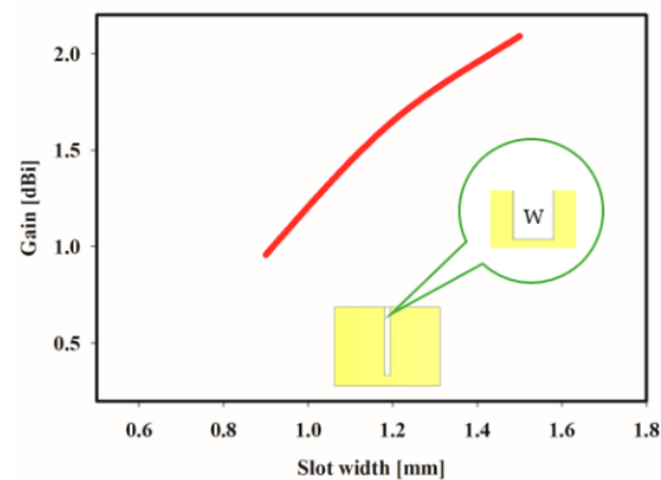
Figure 9. Simulated analysis of gain.
