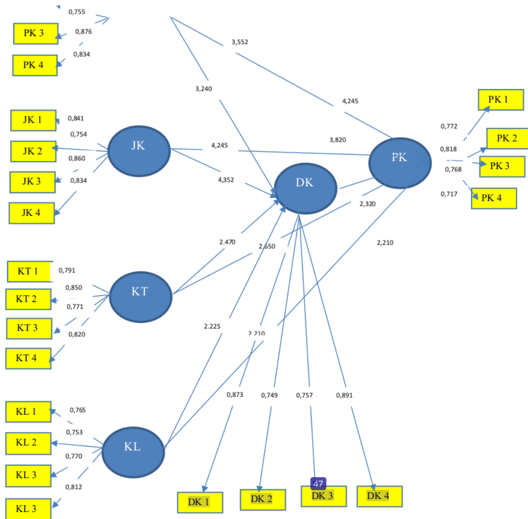
Gambar 1. Diagram Bootstrapping
