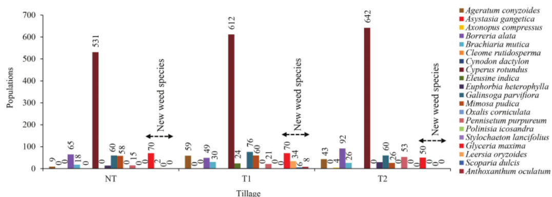
Figure 5. Changes in weed vegetation due to ammonium glufosinate application at a dose of 150 g a.i. ha -1 on different tillage systems (NT: no-tillage; T1: 1-time tillage; T2: 2-times tillage).
