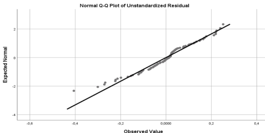
Figure 2 Probability Plot
