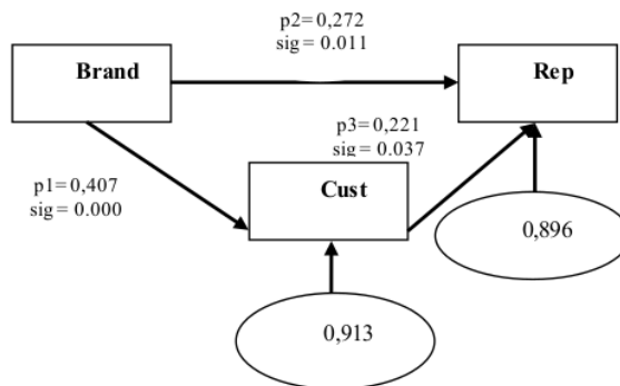
Gambar 2. Model Analisis Jalur (( Path Analysis ))
