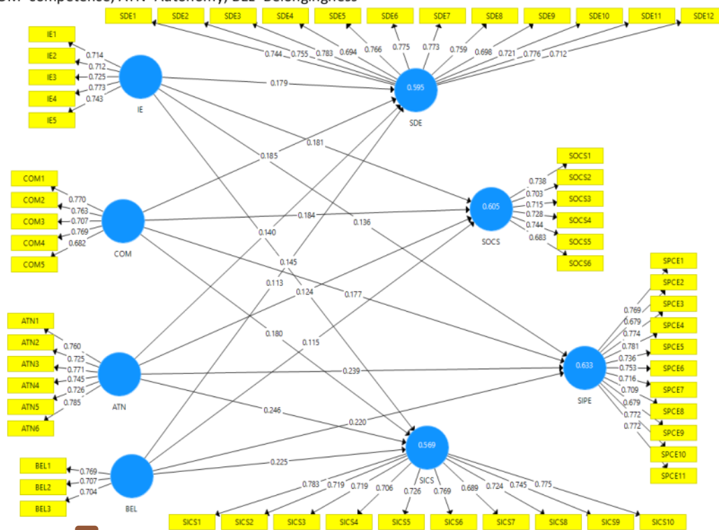
Figure 2: Full Measurement Model
