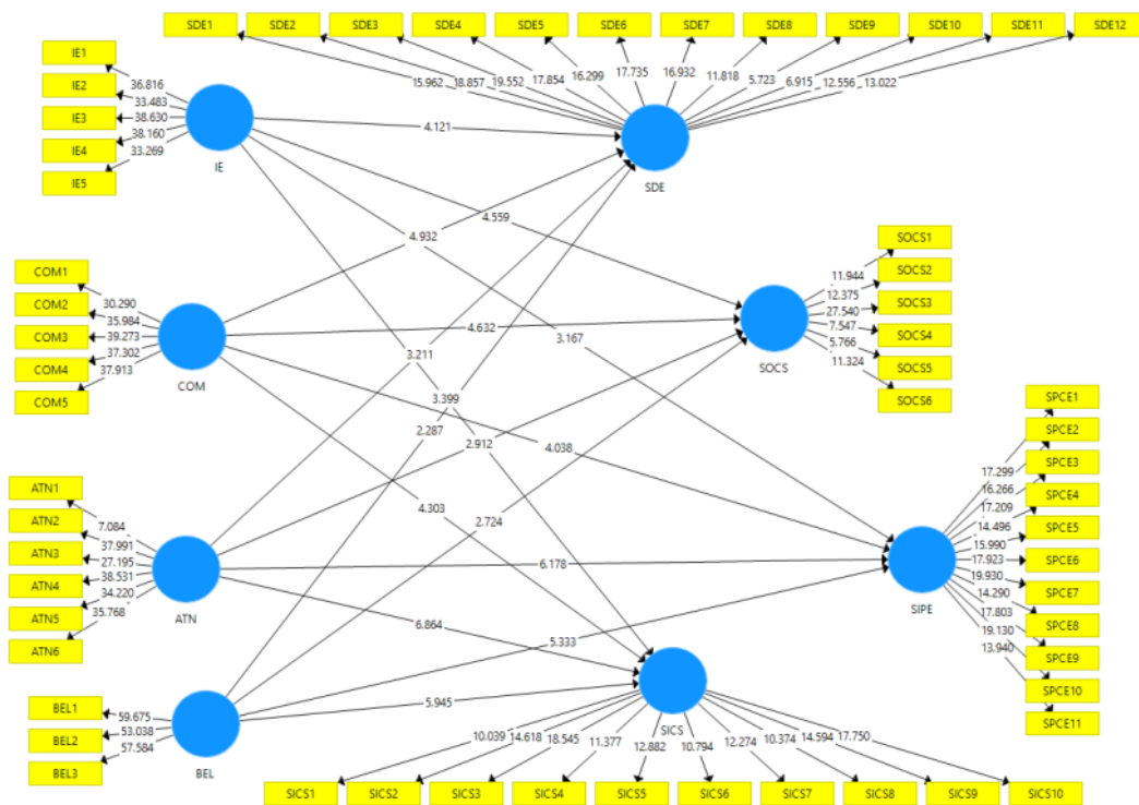
Figure 3: Full Structural Model
