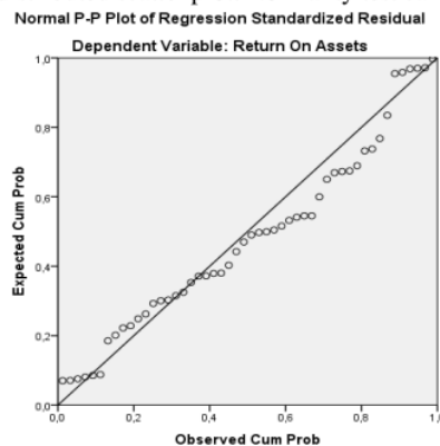
Figure 4.1 P-Plot . Normality Test Results
