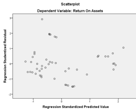
Figure 4.2 Heteroscedasticity Test Results
