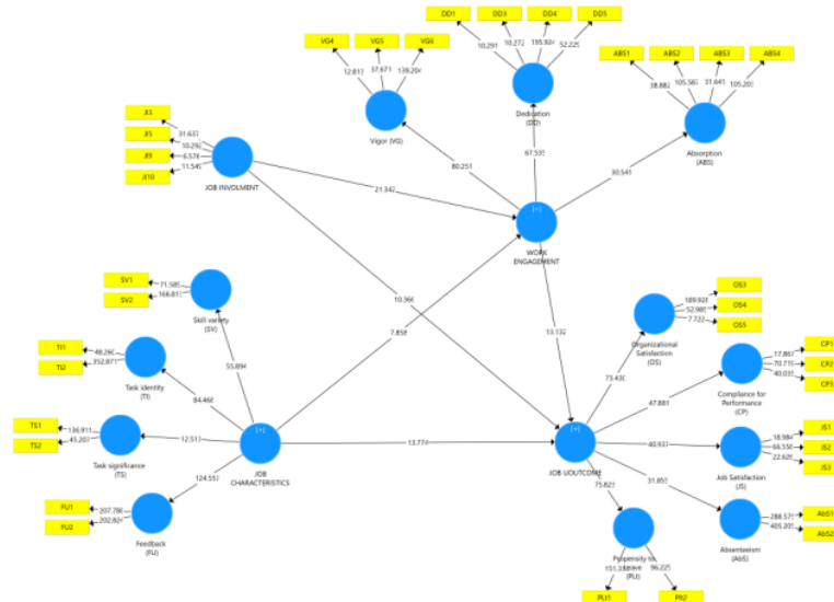
Gambar 3. Model Struktural Penelitian (Inner Model)
