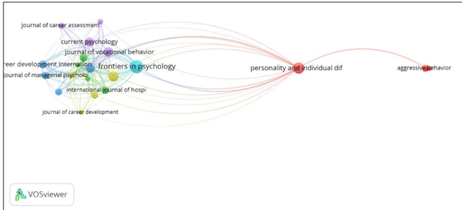
The most cited journals related to proactive personality are the journal of psychology as many as 15 documents with 3880 citations; then frontiers in psychology as many as 32 documents with 192 citations; then personnel psychology as many as six documents with 1333 citations.
