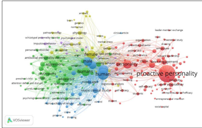
Figure 7. The visualization results of Figure 7 found there are 5 clusters; it can be seen which clusters have the opportunity to be researched in the future that has to do with proactive personality.
