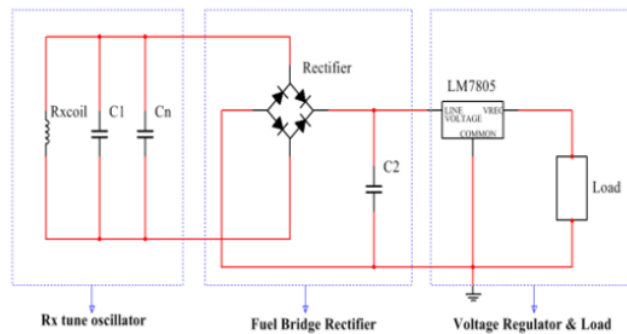
Figure 3: Receiver circuit design
