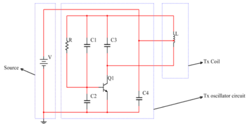
Figure 1: Design of transmitter circuit using one transistor
