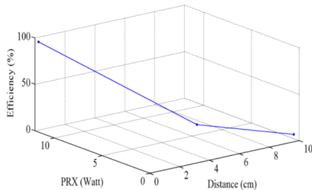
Figure 5: Wireless power transfer using BC639 transistor
