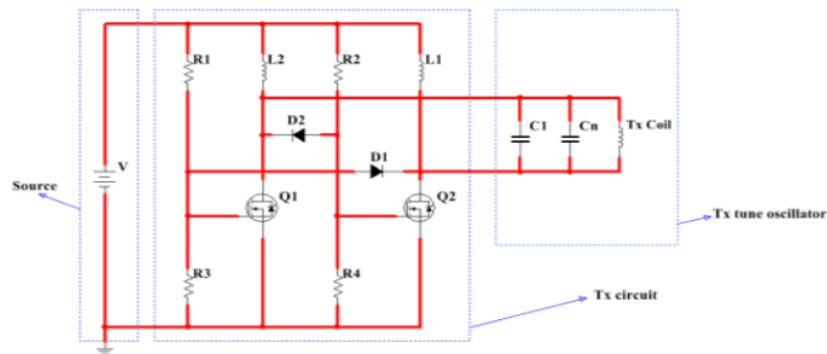
Figure 2: Design of transmitter circuit using parallel MOSFET
