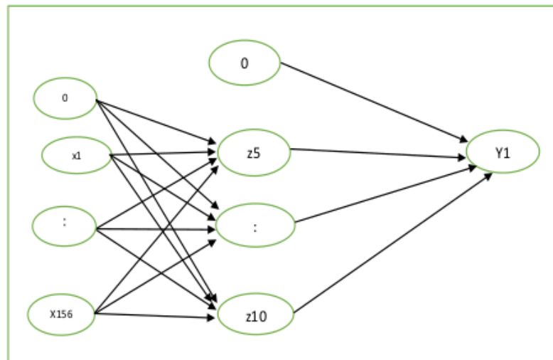
Gambar 1. Model Jaringan Saraf Tiruan Back Propagation
